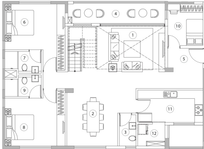
UNIT A DUPLEX LOWER (FLOOR - 10)
