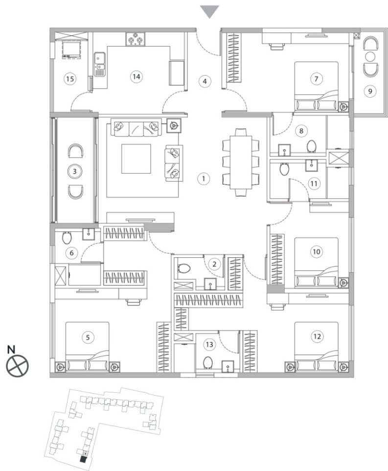
UNIT C SIMPLEX (FLOOR 2 TO 11)
