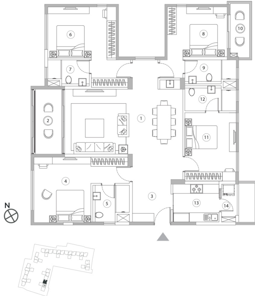
UNIT B SIMPLEX (FLOOR 2 TO 11)
